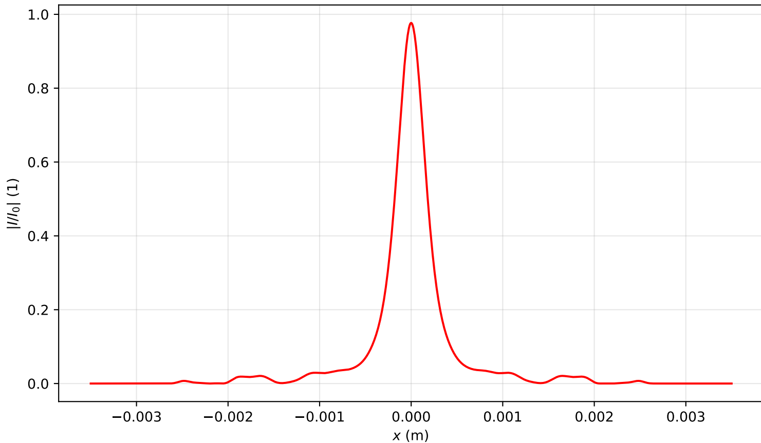
Intensity profile I(x, y = 0, z = 3.105)/I_0 , P_{in}=4.0P_{cr} , artificial time
